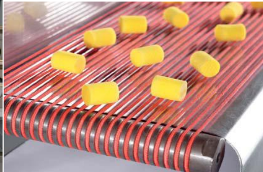
Polyester round belt PVA red in a transport machine
