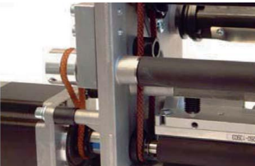
Vulkollan round belt in a label printer
