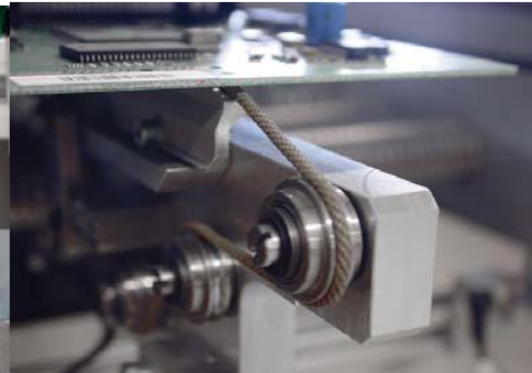
3 mm PBO round belt supporting a circuit board in a soldering machine at 380° C
