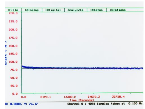
Dynamic force-elongation chart
