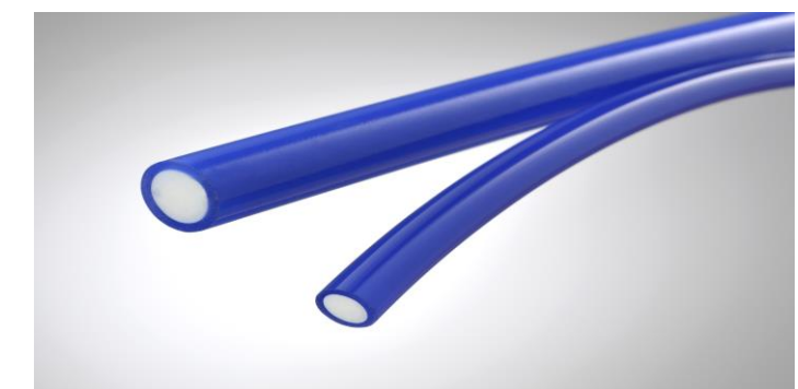
70 Sh.A EU/FDA sheath with 90 Sh.A core
